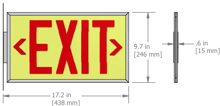
EDGE MOUNTED
